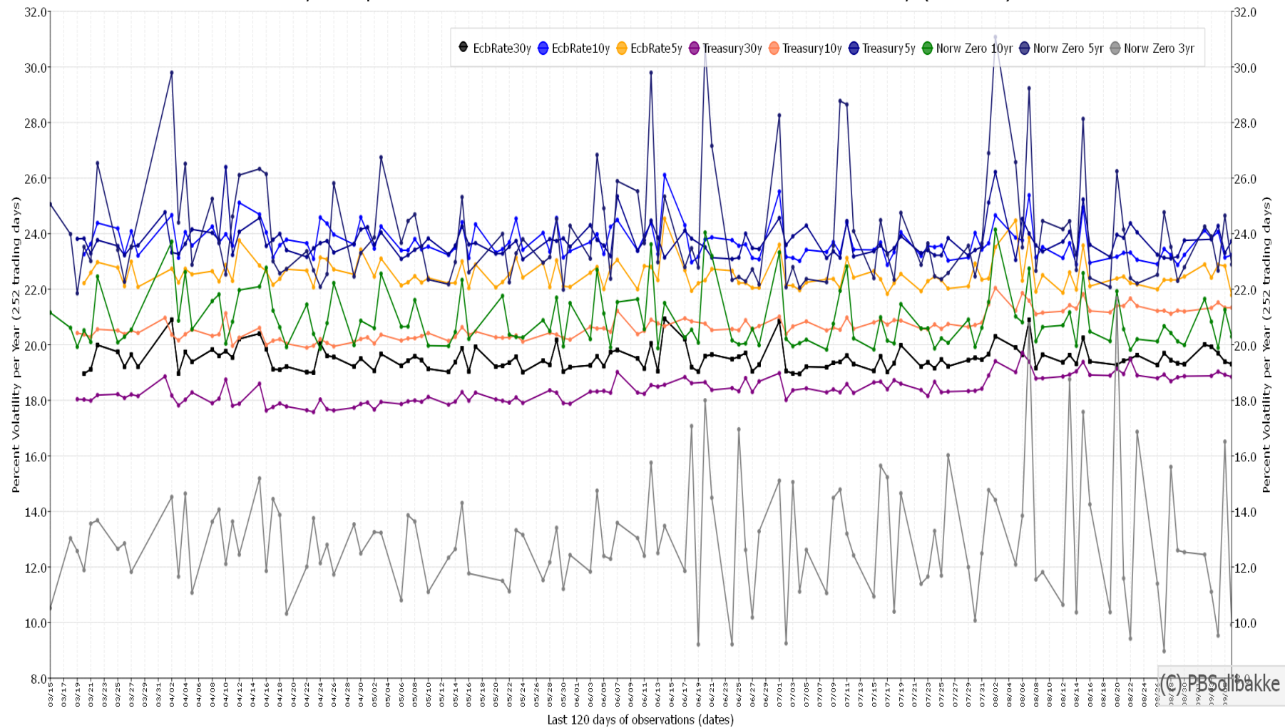
Daily European and US Interest Rates / Bonds: Stochastic Volatility (120 tics)
