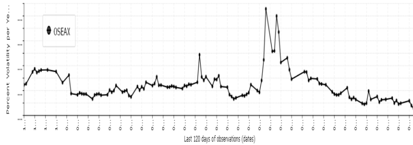
Daily OSEAX (No) Equity Index: Stochastic Volatility (120 tics)
