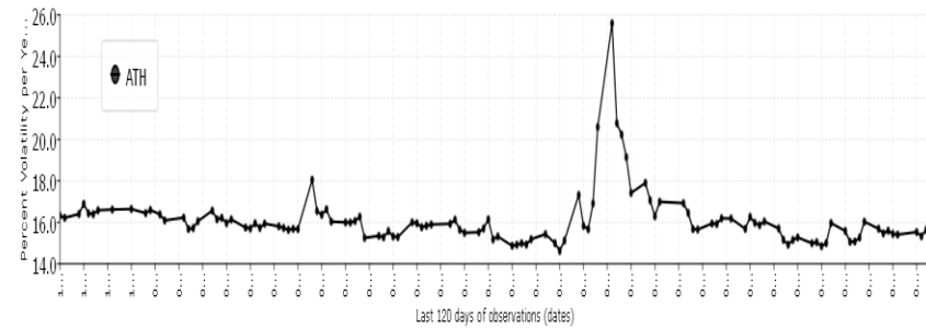
Daily Athen Greece ATH Index: Stochastic Volatility (120 tics)
