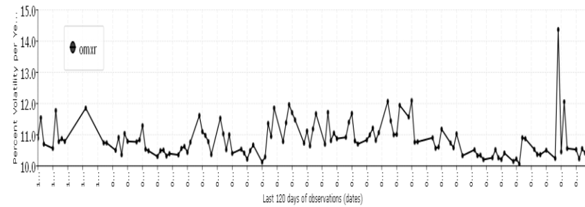
Daily omxr (Riga, Latvia) Index: Stochastic Volatility (120 tics)
