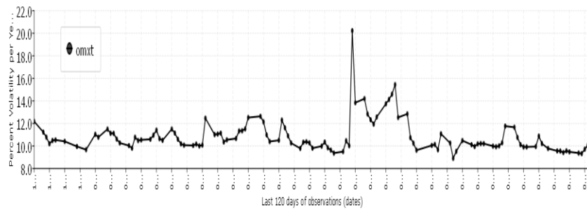
Daily omxt (Tallinn, Litauen) Index: Stochastic Volatility (120 tics)
