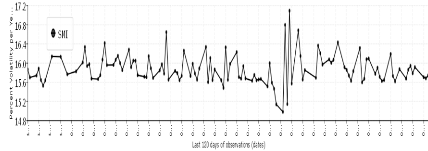
Daily Switzerland SMI Index: Stochastic Volatility (120 tics)
