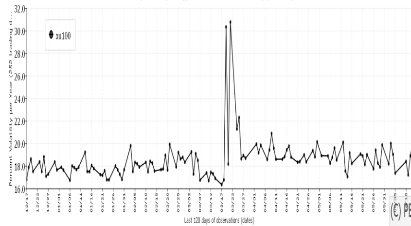
Daily xu100 (Turkey) Index: Stochastic Volatility (120 tics)
