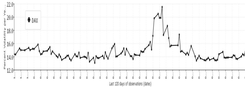
Daily France CAC Index: Stochastic Volatility (120 tics)
