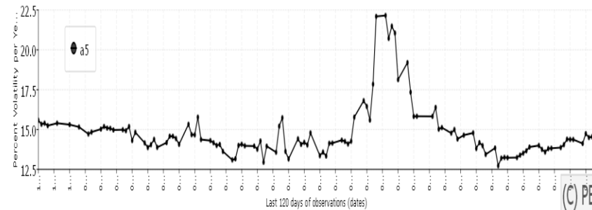
Daily A5 Vienna Index: Stochastic Volatility (120 tics)
