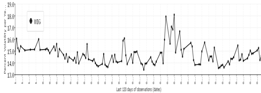
Daily Polen WIG Index: Stochastic Volatility (120 tics)
