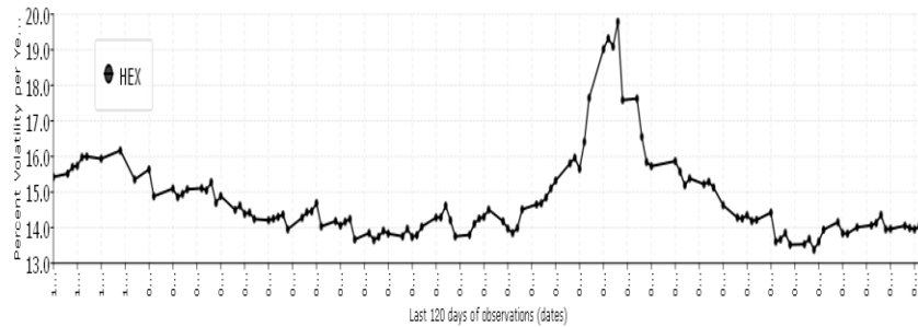
Daily Helsinki Finland HEX Index: Stochastic Volatility (120 tics)
