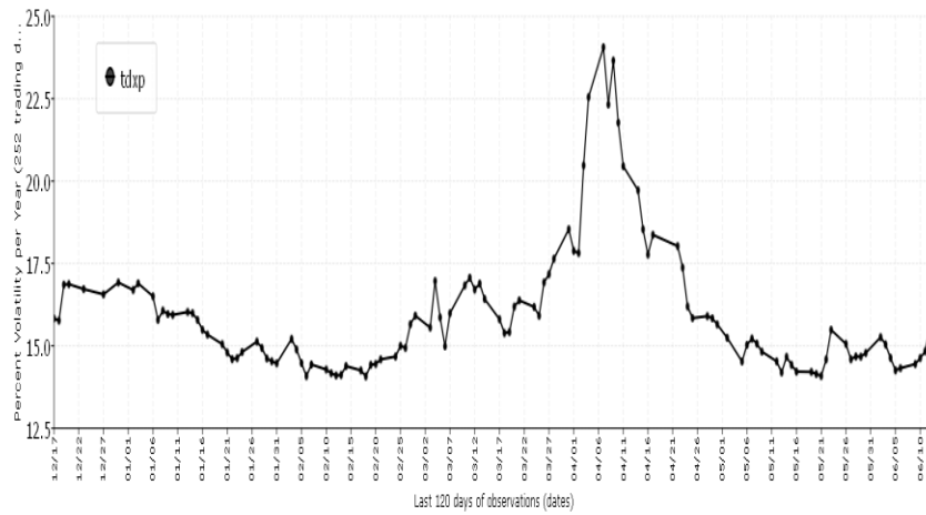
Daily tdxp (Germany) Index: Stochastic Volatility (120 tics)
