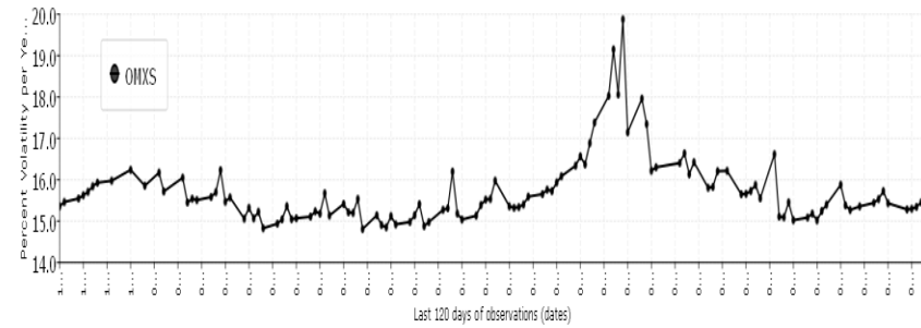
Daily OMXS (Sweden) Index: Stochastic Volatility (120 tics)
