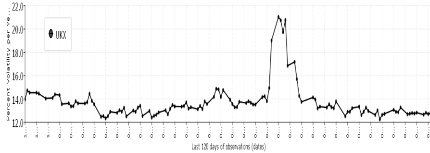
Daily the UK UKX/FTSE100 Index: Stochastic Volatility (120 tics)
