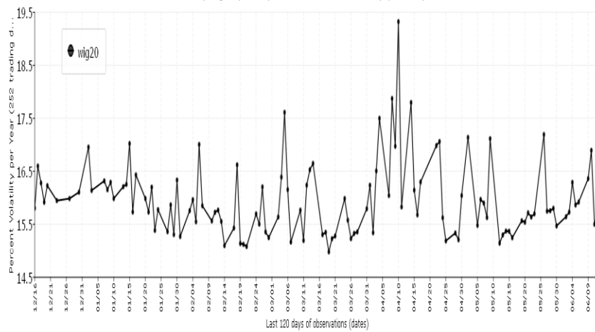
Daily wig20 (Poland) Index: Stochastic Volatility (120 tics)
