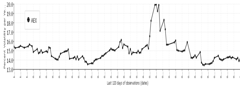
Daily Amsterdam NL AEX Index: Stochastic Volatility (120 tics)
