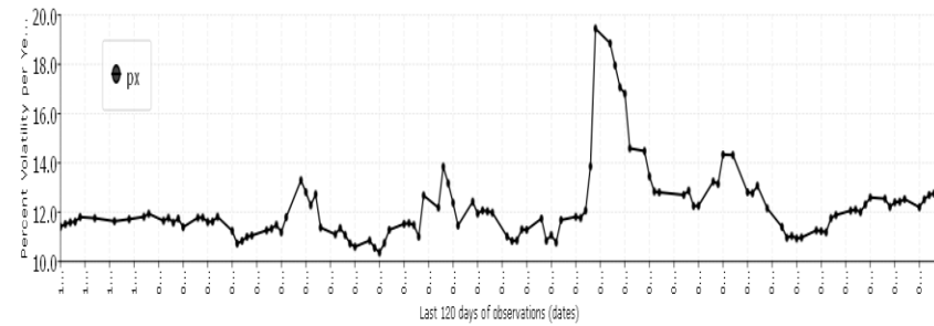
Daily px (xxxxxxx) Index: Stochastic Volatility (120 tics)
