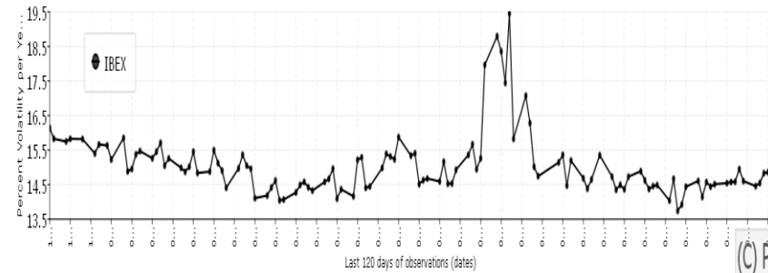
Daily Spain IBEX Index: Stochastic Volatility (120 tics)
