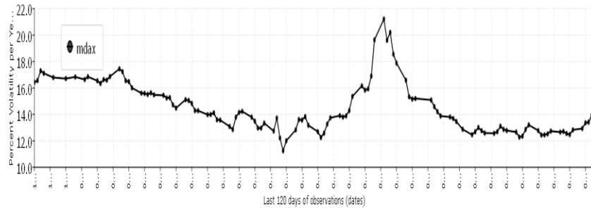
Daily mdax (Germany) Index: Stochastic Volatility (120 tics)
